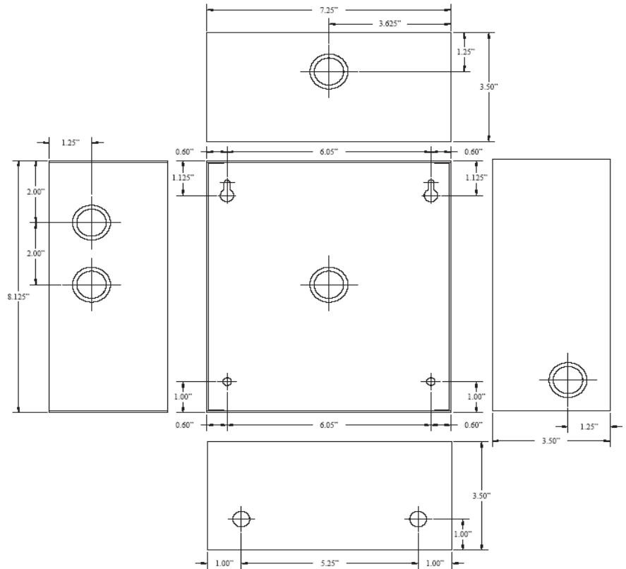
Enclosure Dimensions ( 8.5"H x 7.5"W x 3.5"D)
